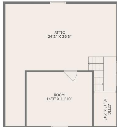
3rd FLOOR
