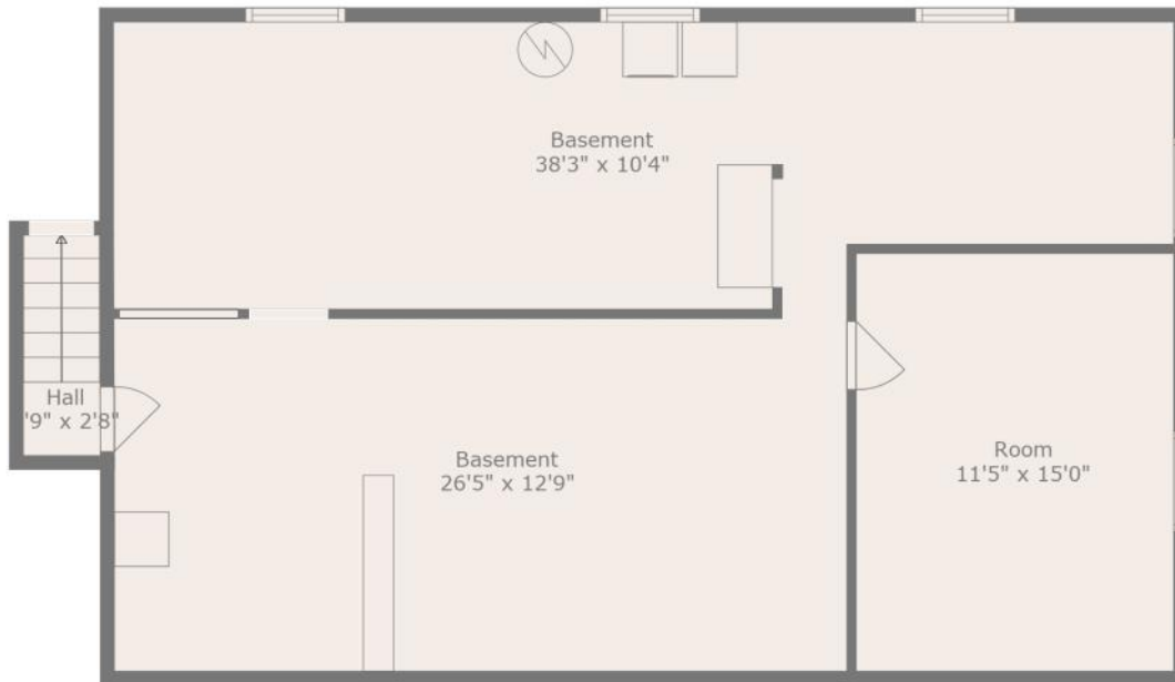
LOWER LEVEL
