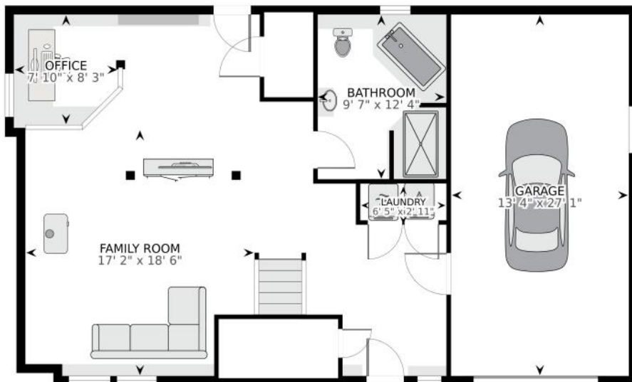
LOWER LEVEL
