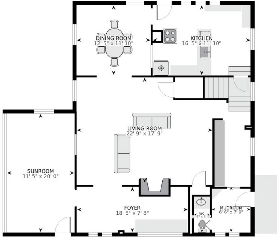
FIRST FLOOR
