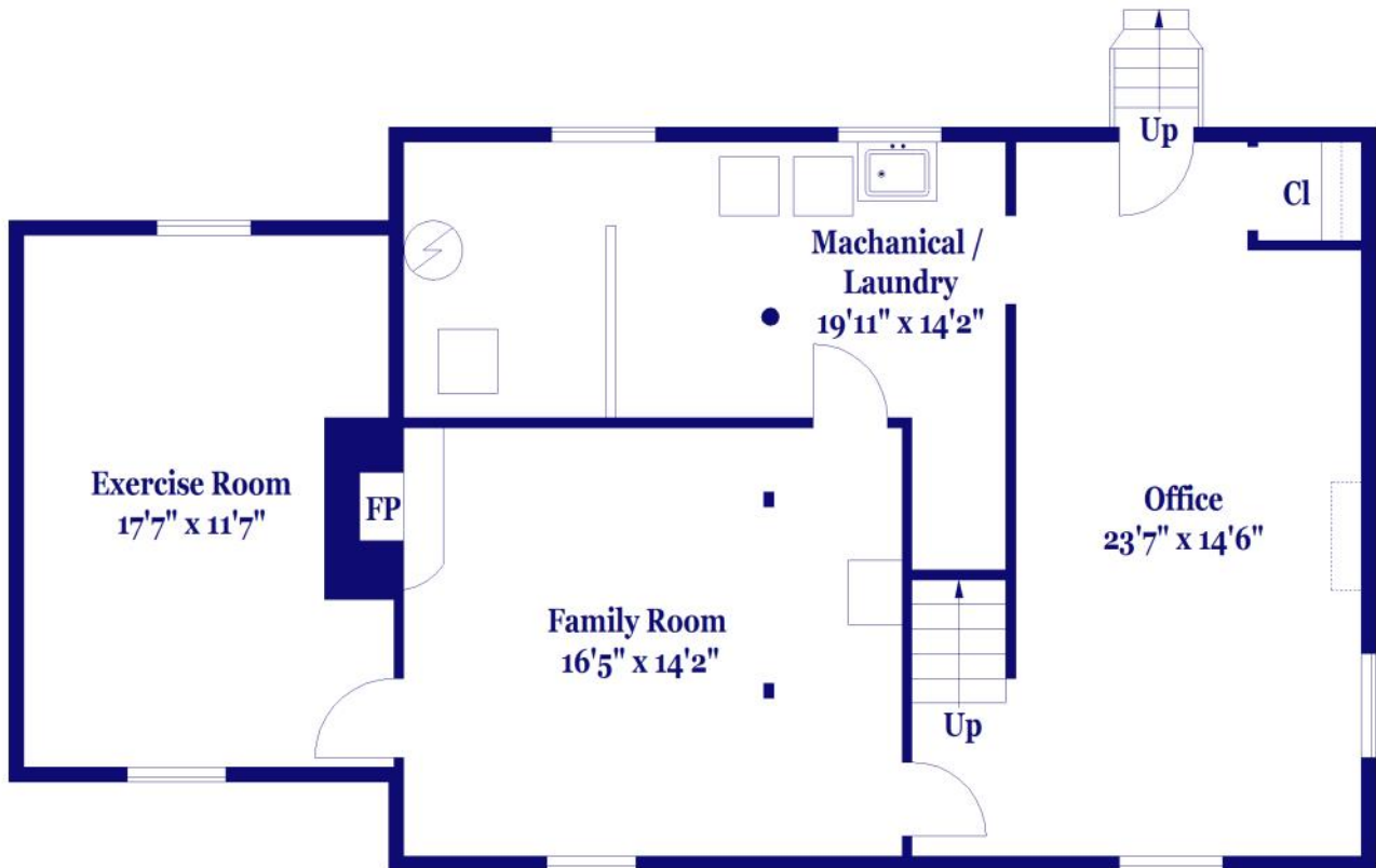
LOWER FLOOR
