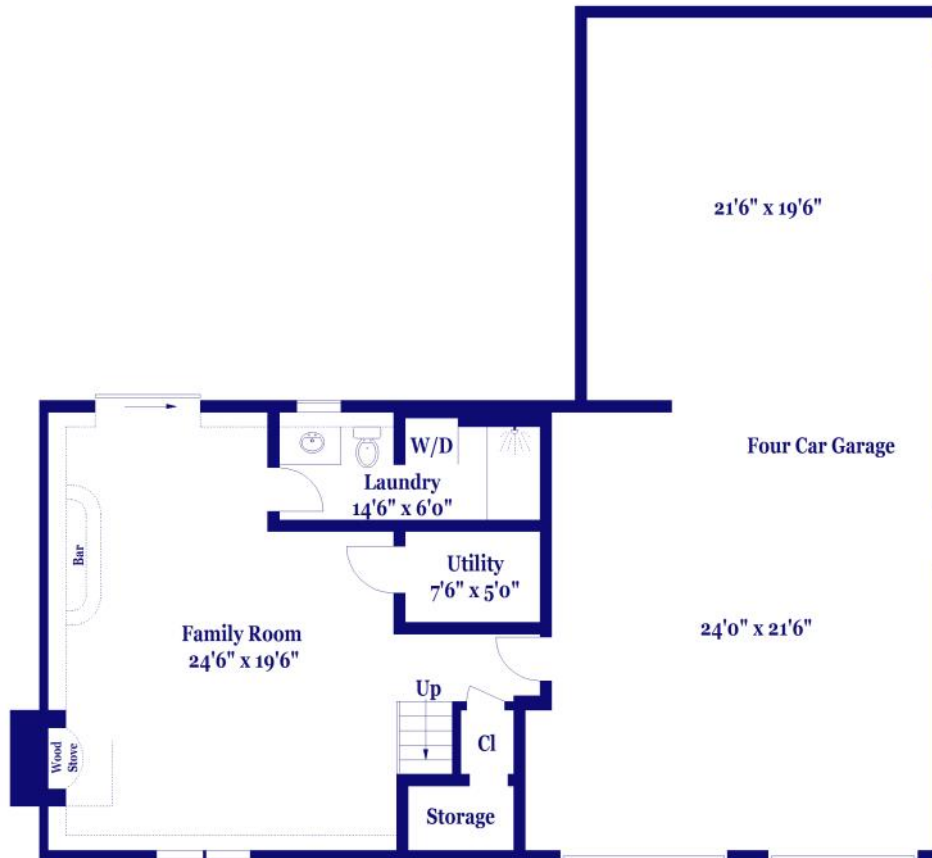
LOWER LEVEL
