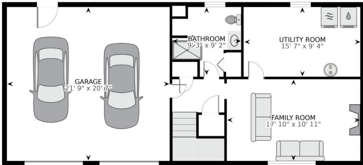
LOWER LEVEL
