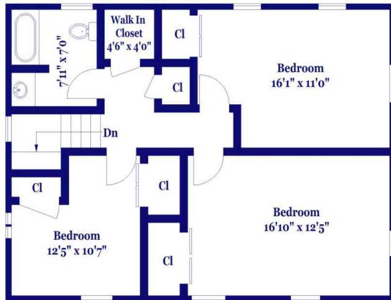
SECOND FLOOR
