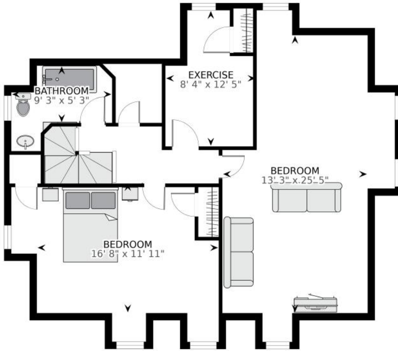
THIRD FLOOR
