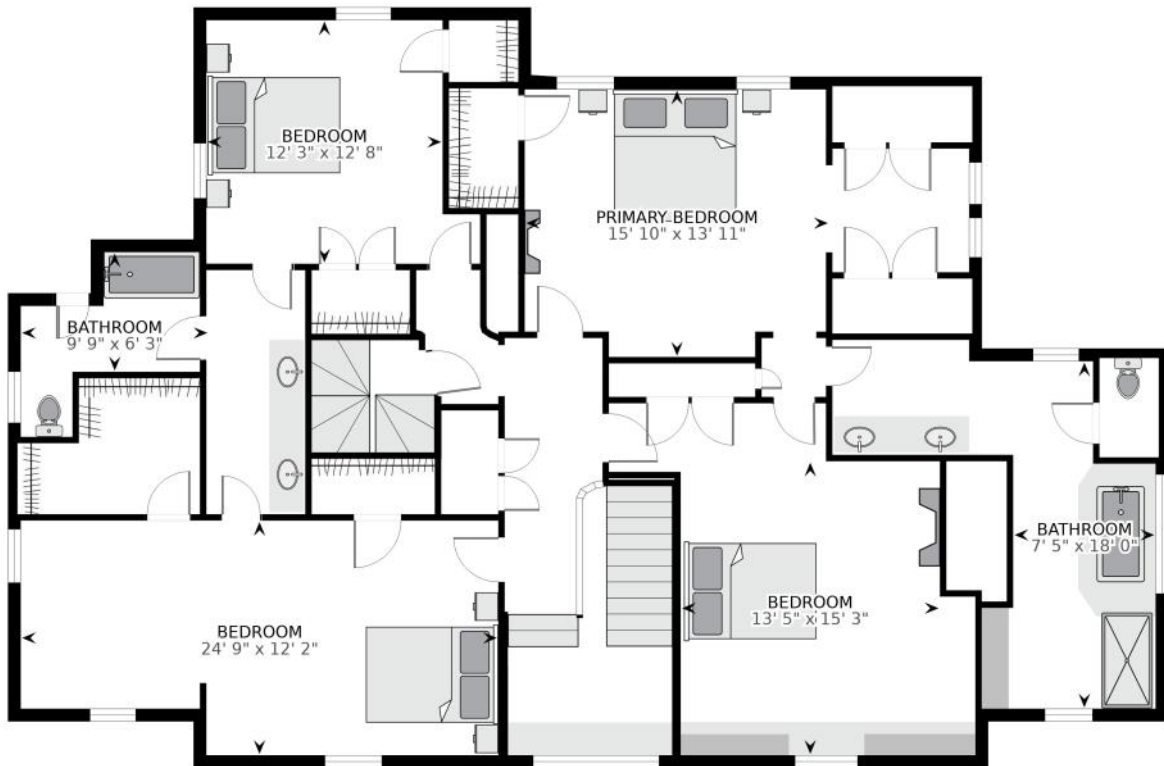
SECOND FLOOR
