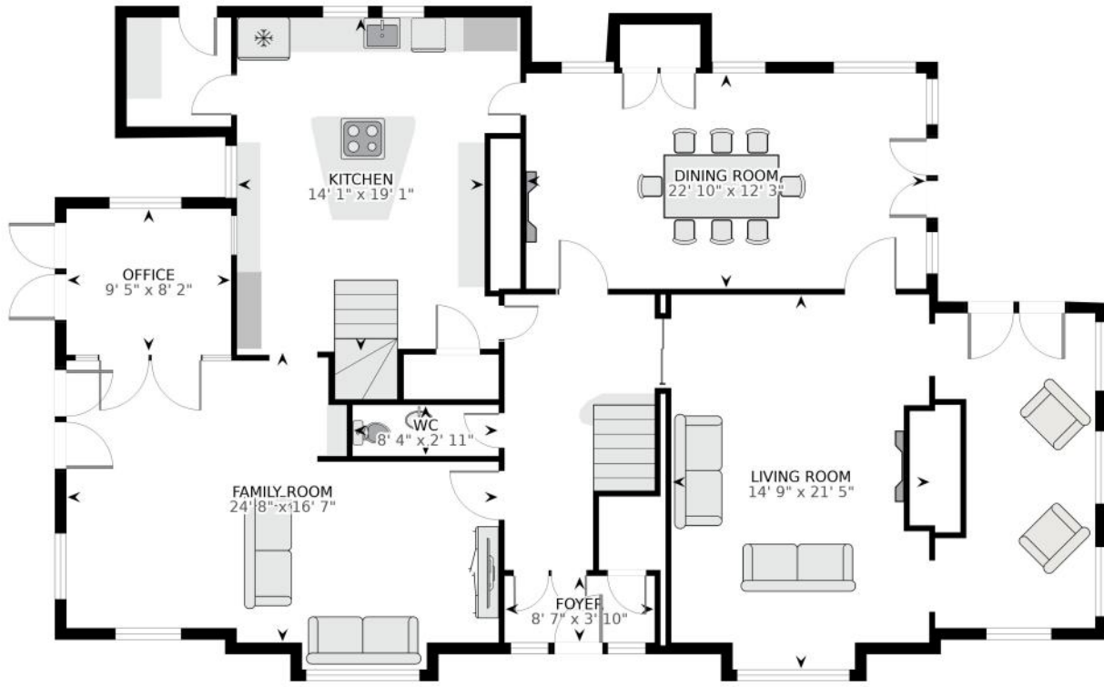
MAIN FLOOR
