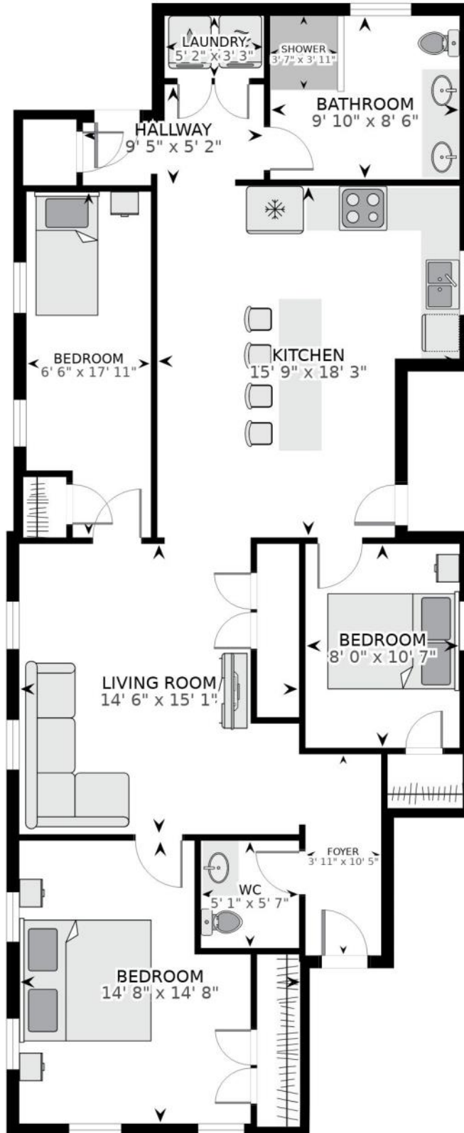
MAIN FLOOR
